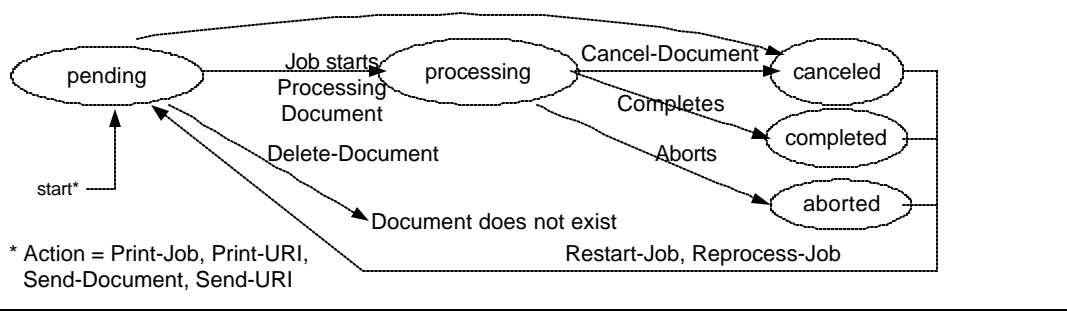
1416 Figure 1 - The "document-state" Document Description attribute and the Document object life cycle
